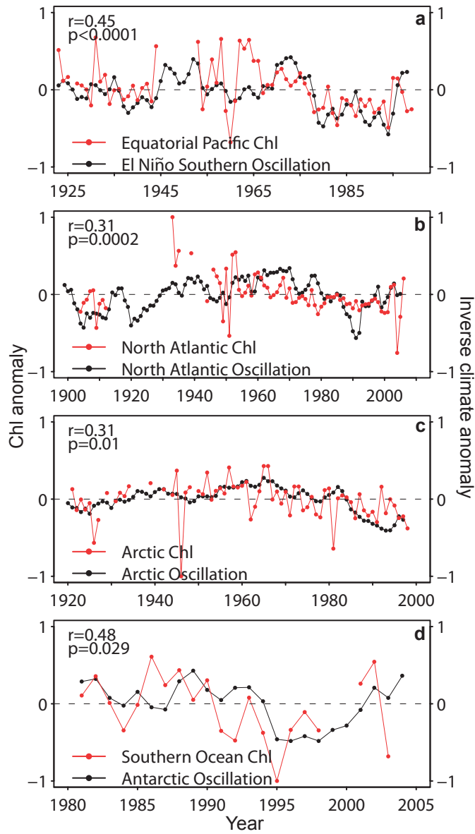
Figure 5 | Effects of climate variability on phytoplankton. (a) Linear relationships between normalized and de-trended yearly Chl anomalies (red) and smoothed climate indices (black) for (a) the Equatorial Pacific, (b) the North Atlantic, (c) the Arctic, and (d) the Southern Ocean regions. Pearson correlation coefficients and p-values are shown. Climate indices and correlation coefficients have been inverted in order to better visualize correlations.
