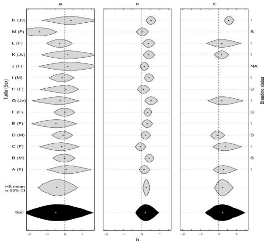
Fig. 3. Raindrop plots (Barrowman & Myers 2003) summarizing the 95% credible intervals of the posterior densities of \hat{\delta}_j , the log ratio of day-to-night travel rates of leatherback turtles during the predominant phases of their migratory cycle: (a) northern foraging, (b) southward migration and (c) northward migration. The sex and breeding status (where known) of each turtle are displayed on panels (a) and (c), respectively. The point within each raindrop indicates the posterior mode. The taller raindrops in the bottom two rows of the panels are hierarchical summaries, and are interpreted differently from the raindrops for the individual turtles. The ‘mean w 95% CI’ raindrops are the estimated hierarchical means \hat{\mu}_{\delta} with 95% credible intervals. The raindrops for the Bayes predictive distributions (Bpd) are shaded in black to emphasize that they are different from the mean. These distributions summarize all the information available to predict \delta_j for an unobserved turtle.
