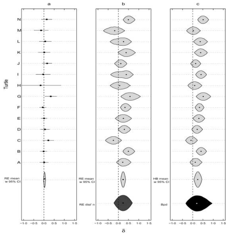
Fig. 5. Comparison of \hat{\delta}_j , the log ratio of day-to-night travel rates for (a) a conventional calculation of travel rates from ad hoc filtered data, (b) non-hierarchical state–space model estimates of \delta_j and (c) hierarchical state–space model estimates of \delta_j . The results presented are for the southward migratory segments only. The ratios presented in (a) are means with 95% confidence intervals, and those presented in (b) and (c) are posterior modes with 95% credible interval raindrops. Note there is no random effects variance presented in (a) because the estimate was 0.
