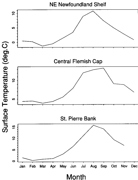
Figure 7. Monthly mean surface temperatures (°C) for three representative areas.
