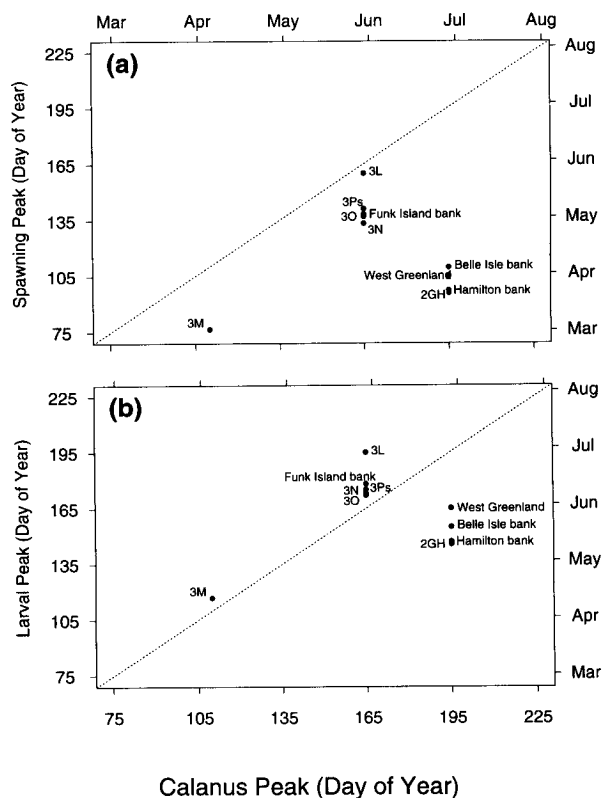
Figure 6. (a) Mean spawning time versus the date of the peak for Calanus finmarchicus I–IV. The dashed line indicates direct proportionality with unit slope. (b) Estimated time of appearance of first-feeding larvae versus the date of the peak for Calanus finmarchicus I–IV. The dashed line indicates direct proportionality with unit slope.
