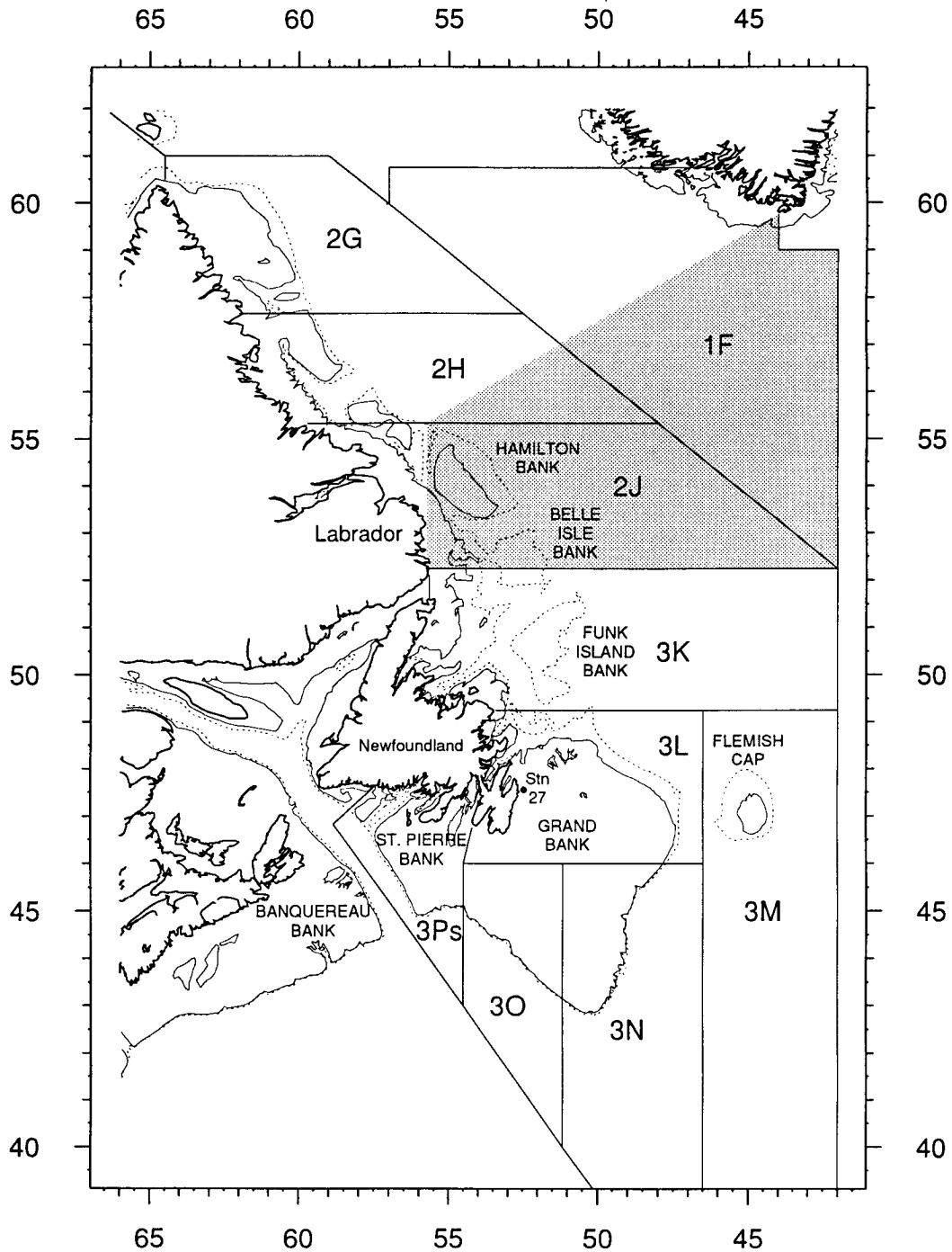
Figure 1. Map of the study region, with the NAFO zones. Funk Island Bank and Belle Isle Bank are conveniently delineated by the 300 m isobath, as indicated here (dashed line). The stippled areas of Regions 1 and 2 indicate the portions of these zones for which continuous Plankton Recorder (Robinson et al. , 1973) coverage was available.
