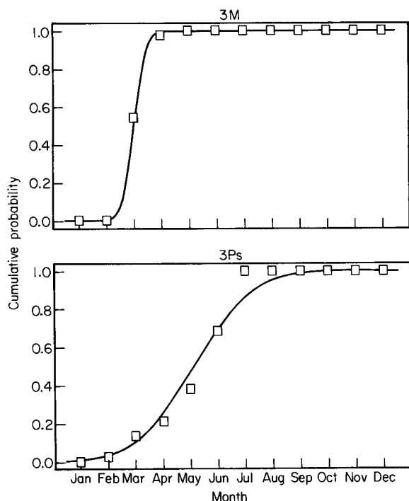
Figure 2. Fitted maturity ogives for two extreme cases: zone 3M (very narrow spawning window); zone 3Ps (very wide spawning window). The squares designate the monthly proportions of the female fish that are spent.
