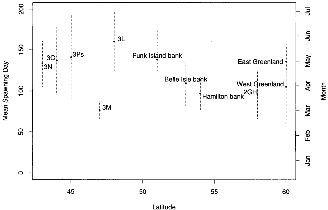
Figure 4. The latitudinal dependence of mean spawning time. The dotted lines indicate the widths (standard deviations) of the spawning distributions.
