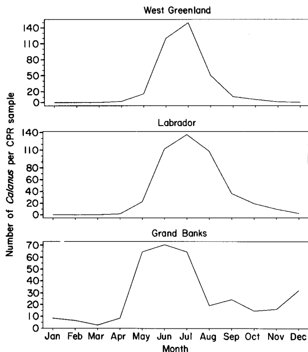
Figure 5. Plots of the estimated abundance (based on CPR data) of Calanus finmarchicus I–IV for West Greenland (Region 1), Labrador (Region 2) and the Grand Bank (Region 3) waters, from Robinson et al. (1973).
